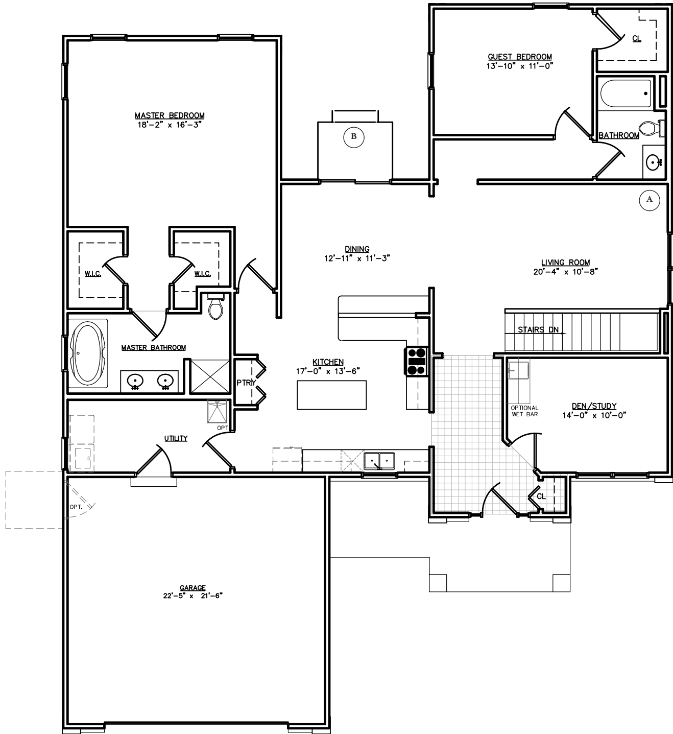
Standard Floor Plan
