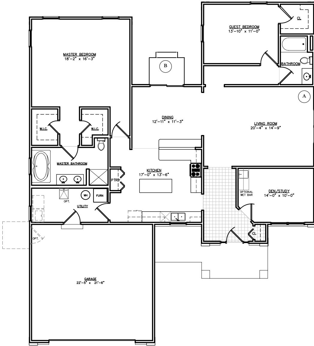
Standard Floor Plan
